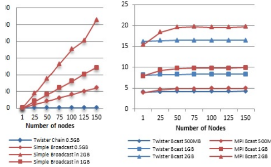
Figure 5. Twister Chain vs. Simple Broadcasting
