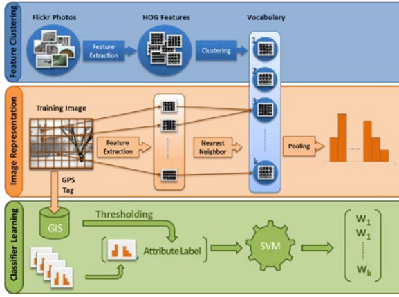
Figure 1. Workflow of the vocabulary learning application.
