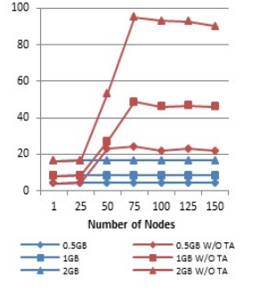
Figure 9. Twister Chain with/without topology-awareness
