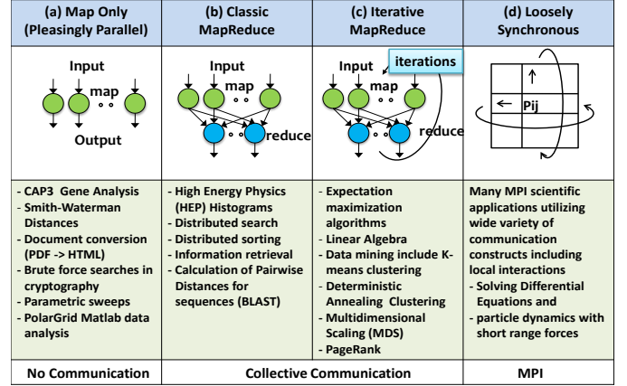
Figure 3. Classification of Applications
