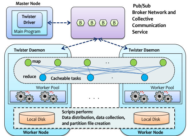
Figure 4. Initial Twister architecture
