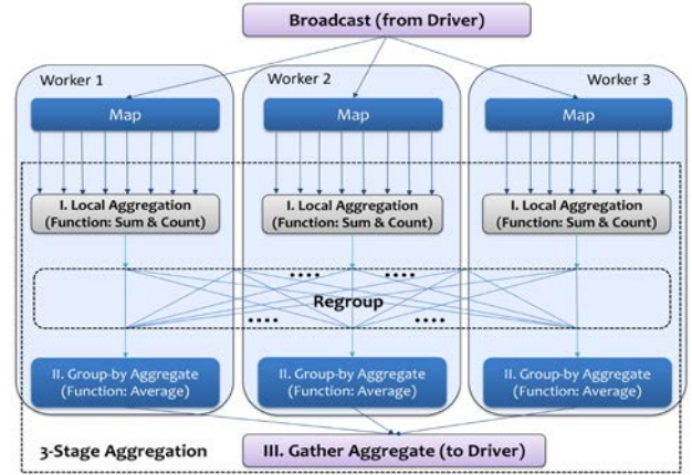
Figure 2. Image clustering control flow in Twister with the new local aggregation feature in Map stage.
